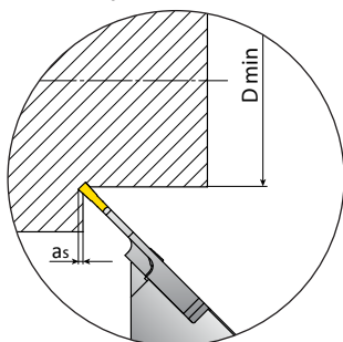
Square Groove
