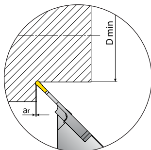
Round Groove
